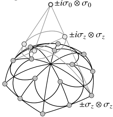
Figure 3: Q_4(2) , its nucleus, and a portion of its ambient space as the geometry behind the complex two-qubit Pauli group.
