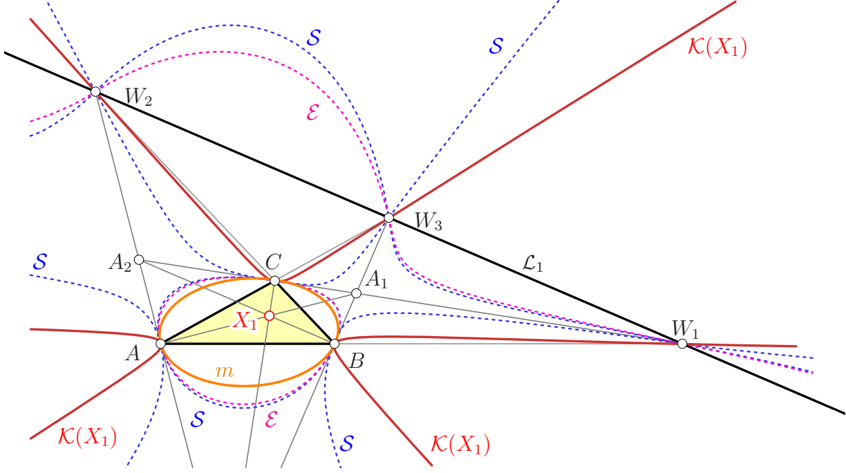
Figure 4: The side lines of \Delta and \Delta_e are degenerate permutation cubics. The cubic \mathcal{K}(X_1) is the only rational permutation cubic. The elliptic sextic \mathcal{S} and the elliptic cubic \mathcal{E} are artifacts of the computation.
