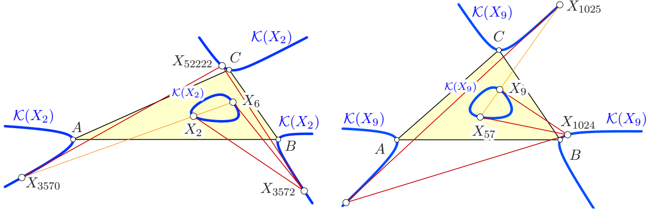
Figure 6: Two permutation cubics: \mathcal{K}(X_2) (left) and \mathcal{K}(X_9) (right) with some centers on them.
