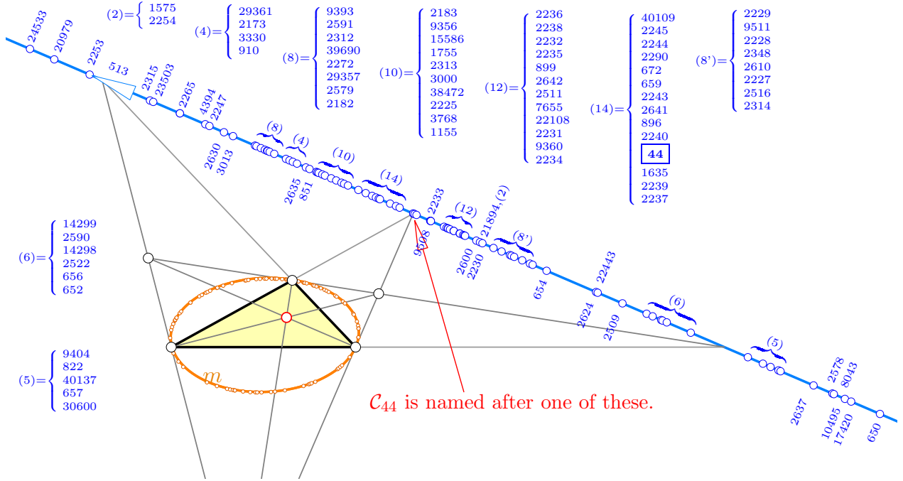
Figure 8: The straight part \mathcal{L}_1 of \mathcal{K}(X_{44}) with some triangle centers on it.
