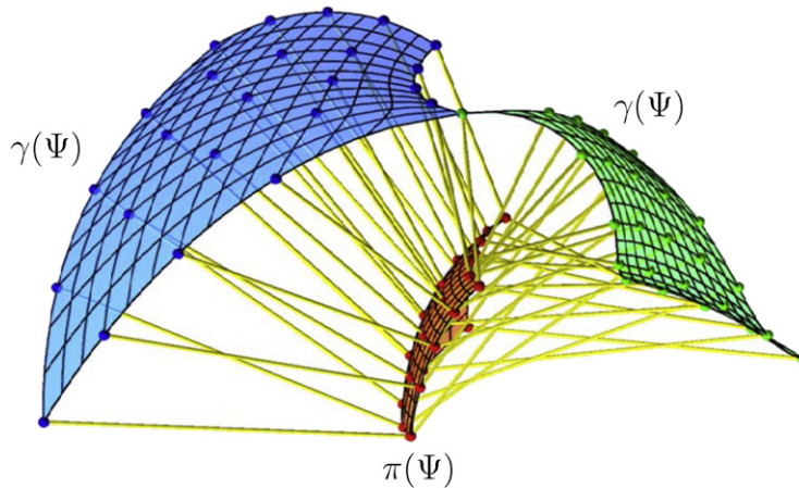
Fig. 8. Rational envelope \gamma(\Psi) and top view \pi(\Psi) of a surface \Psi \in \mathbb{R}^4 .
