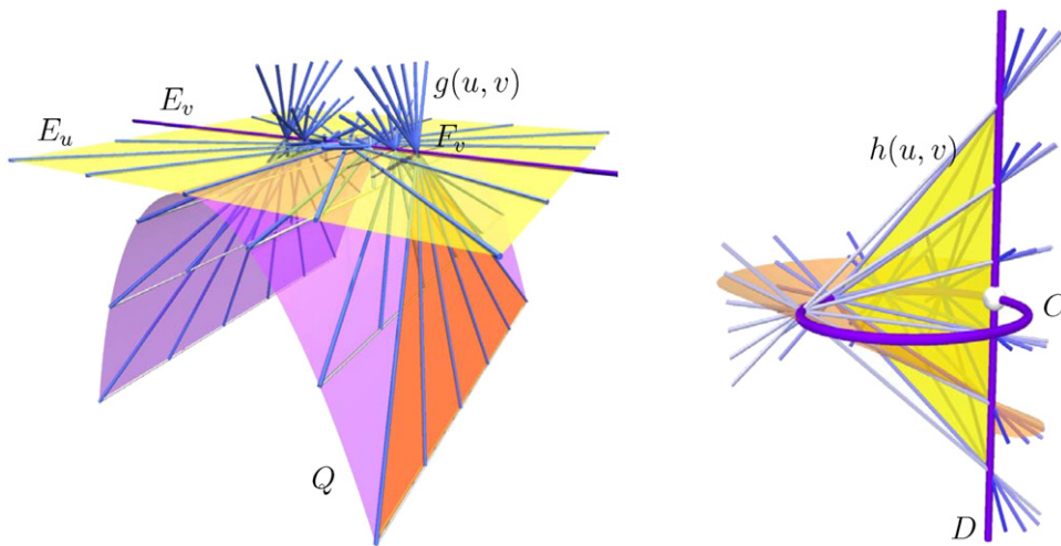
Fig. 5. Left: Family of lines \mathcal{G} from case 4. Right: Family of lines \mathcal{H} from case 4.
