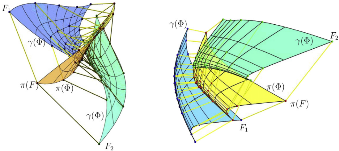
Fig. 7. Cyclographic images \gamma(\Phi) and orthogonal projection \pi(\Phi) of quadratic triangular Bézier surfaces \subset \mathbb{R}^4 . Left: Example 1. Right: Example 2.
