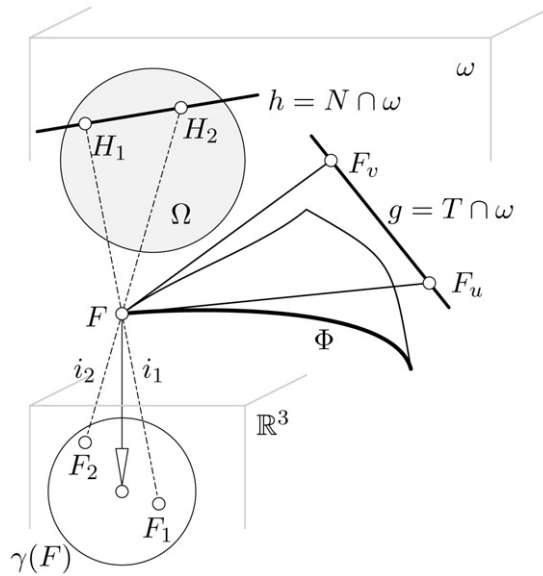
Fig. 3. Construction of the cyclographic image from the projective point of view.
