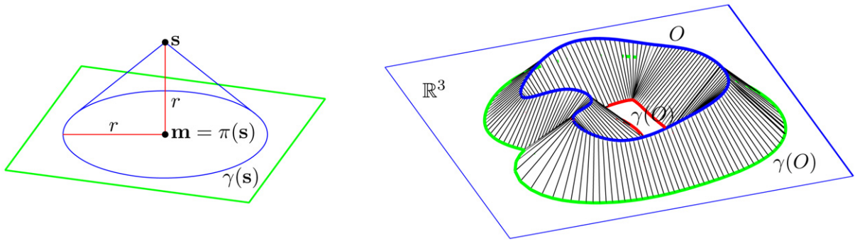
Fig. 1. Left: Cyclographic mapping \gamma : \mathbb{R}^3 \rightarrow \mathbb{R}^2 . Right: Cyclographic image \gamma(O) \in \mathbb{R}^2 of curve O \subset \mathbb{R}^3 .
