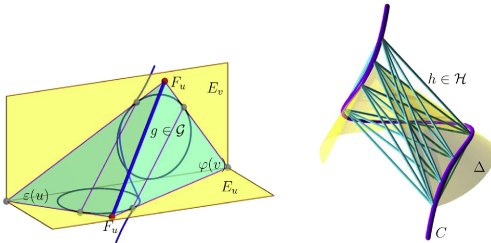
Fig. 6. Left: Axis variety \mathcal{G} . Right: Chordal variety \mathcal{H} of a spatial cubic C .
