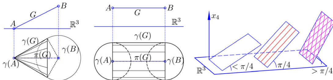
Fig. 2. Left and middle: Cone and cylinder of revolution as cyclographic image of a line \subset \mathbb{R}^4 . Right: Three types of planes and their isotropic directions.
