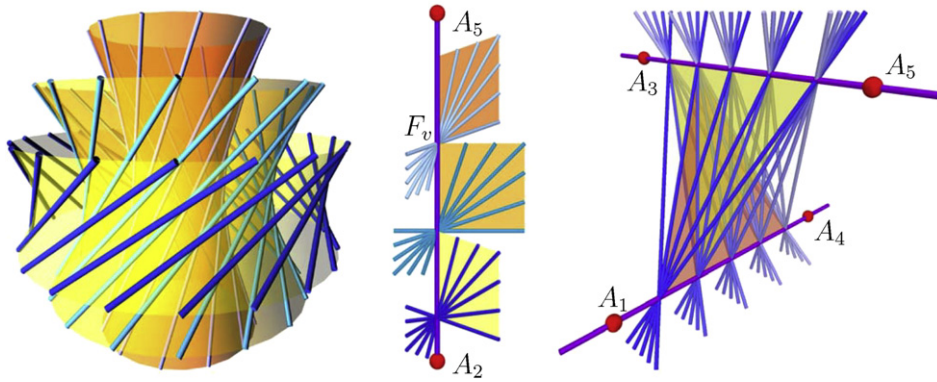
Fig. 4. Three types of linear line congruences in \mathbb{P}^3 . Left: the elliptic type. Middle: the parabolic type. Right: the hyperbolic type.
